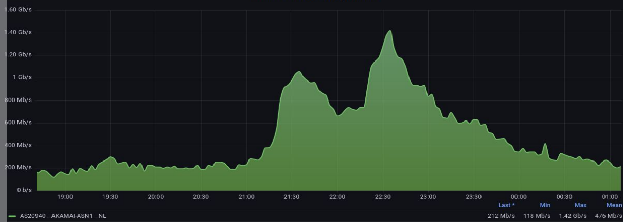
Incoming interfaces
