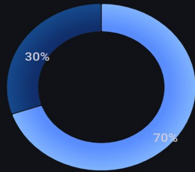
Incoming Routers
